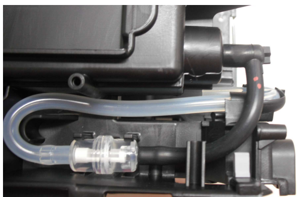
Chassis with new modification p/n 5513216731
